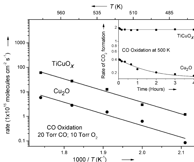
Figure 5. Arrhenius plot of the CO oxidation on \text{Cu}_2\text{O} and \text{TiCuO}_x (ca. 0.6 ML Ti) films. Inset: Catalyst stability during a reaction at 500 K.
